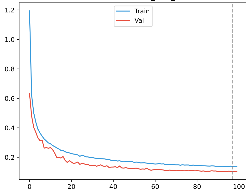
BiLSTM Loss — CIC_IIoT_2025
