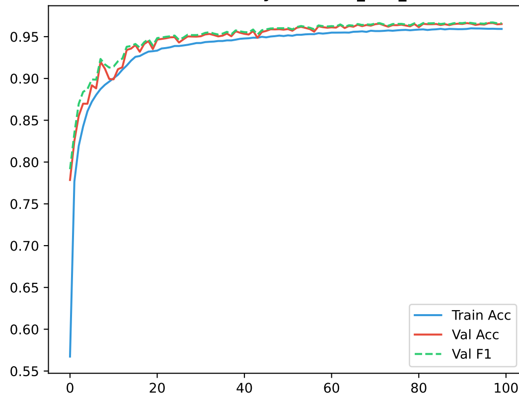
BiLSTM Accuracy/F1 — CIC_IIoT_2025
