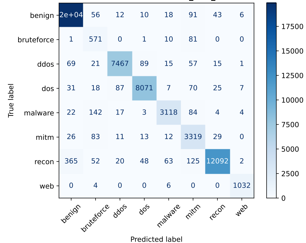
BiLSTM Confusion — CIC_IIoT_2025
